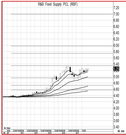
Price Chart...(RBF)
