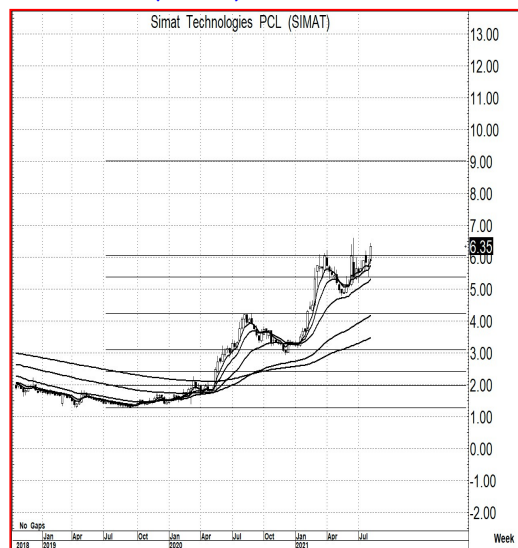
Price Chart...(SIMAT)
