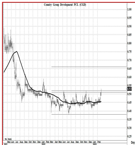
Price Chart...(CGD)
